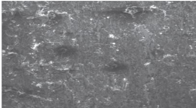
Figure 3 b) sem image of the composite (7.5%SiC, 2.5%TiC, 2%Y 2 O 3 )
